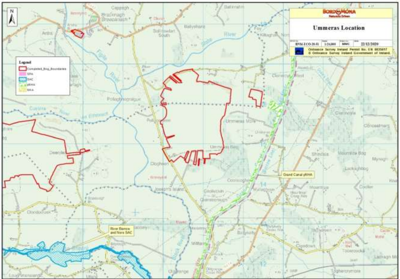
Figure 3.1 Location of Ummeras Bog in context to other Bord na Móna bogs and surrounding area.
