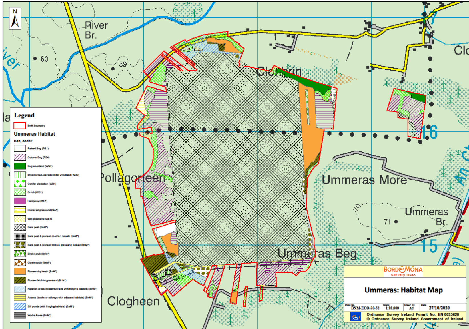
Figure 3.4 Habitat map of Ummeras Bog showing Bord na M6na habitat categorisation
